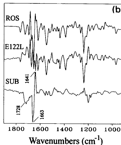
Fig. 5. FT-IR difference spectra. (A) Rho \rightarrow Meta II FT-IR difference spectra of ROS and recombinant mutant rhodopsins (all at 8 \text{cm}^{-1} resolution) measured at 10° C. Each spectrum shown is the average of 3000 scans (10 min) before and after illumination by white light through a 500 nm long-pass filter. (B) Rho \rightarrow Meta II FT-IR difference spectra of ROS and the mutant E122L and their subtraction (SUB: ROS-E122L). The subtracted spectrum shows the missing bands at 1728, 1663 and 1641 \text{cm}^{-1} which are characteristic of the E122L mutation.
