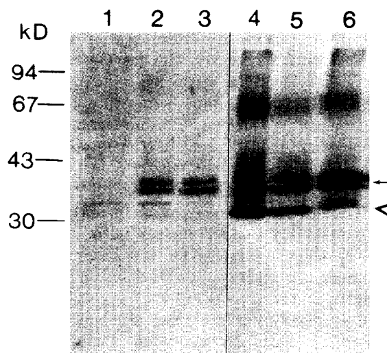
Fig. 1. Immunoblot analysis of Sf9 cells infected with wild-type or mutant recombinant opsin virus (MOI \approx 10). Lanes: 1, wt virus (AcNPV); 2, wt opsin; 3, D83N; 4, E122L; 5, E134D; 6, E134R. Lanes represent approximately 1 \cdot 10^5 cells. Total cell extracts (3 dpi) were separated on a 12% polyacrylamide gel and blotted onto nitrocellulose following standard procedures. Opsin was identified by incubation with antiserum CERNJS858 [31] (dilution 1:1000) followed by standard incubation with HPO-labeled antibodies and assay for HPO activity [11].
