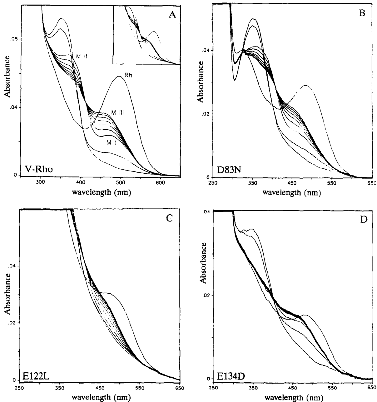
Fig. 3. Late photointermediate formation in reconstituted wild-type and mutant rhodopsins in membrane suspension at pH 6.5. (A) wild-type v-rho. The absorbance bands of rhodopsin (Rh; 498 nm), metarhodopsin I (M I; 480 nm), metarhodopsin II (M II; 380 nm), metarhodopsin III (M III; 455 nm) are indicated in the wild-type v-rho photolysis. (Inset) Photolysis of reconstituted native bovine rhodopsin under similar conditions (3 nmol rhodopsin); (B) D83N; (C) E122L; (D) E134D.
